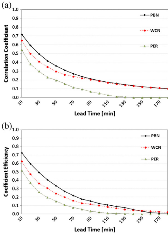
Fig. 10. (a) Correlation Coefficient ( C ) average for ten storms vs. lead time [min]. (b) Coefficient of Efficiency ( E ) average for ten storms vs. lead time [min], both PBN and WCN algorithms, in which the larger values represent better prediction. Three models: PBN, WCN, and PER.
