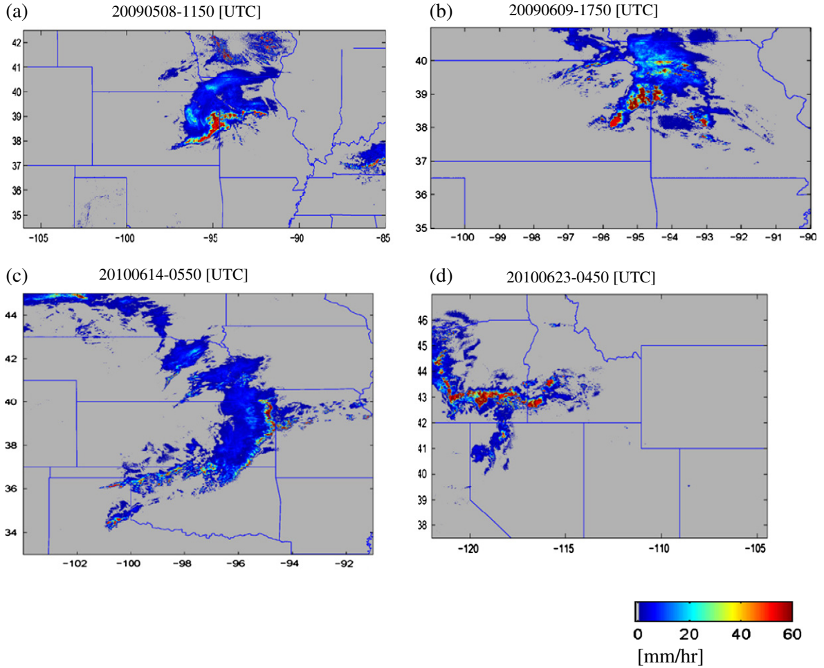
Fig. 5. Four selected severe storms: (a) Event 1:20090508–1150 [UTC], (b) Event 2: 20090609–1750 [UTC], (c) Event 3: 20100614–0550 [UTC], and (d) Event 4: 20100623–0450 [UTC], along with the spatial domain in which the storms produced significant rainfall (Rainfall Unit = mm/hr).
