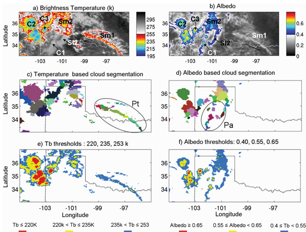
FIG. 3. Demonstration of cloud patches and different threshold layers for an event at 1915 UTC 6 Jul 2006: (a) map of IR Tb, (b) map of smoothed albedo, (c) IR temperature-based cloud patches, (d) albedo-based cloud patches, (e) IR temperature threshold layers, and (f) albedo threshold layers. Cloud-type labels in (a) and (b) are obtained through comparison with Fig. 4. The zones Pt and Pa, shown in (c) and (d) are examples of patches captured by one cloud-patch segmentation approach and not by the other.
