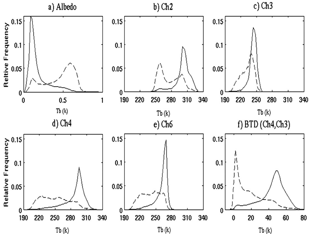
FIG. 7. (a) Relative frequency distributions of albedo, (b)–(e) T_b , and (f) BTD under rain (dashed line) and no-rain (solid line) conditions.
